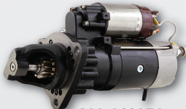
200-46205A 24V, 7.2kW, 12T, CW, INS. with IMS
