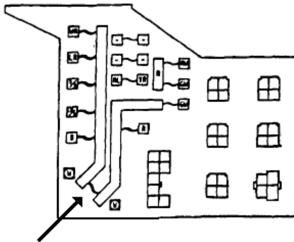
Alternator Circuit Sub-fusible link
